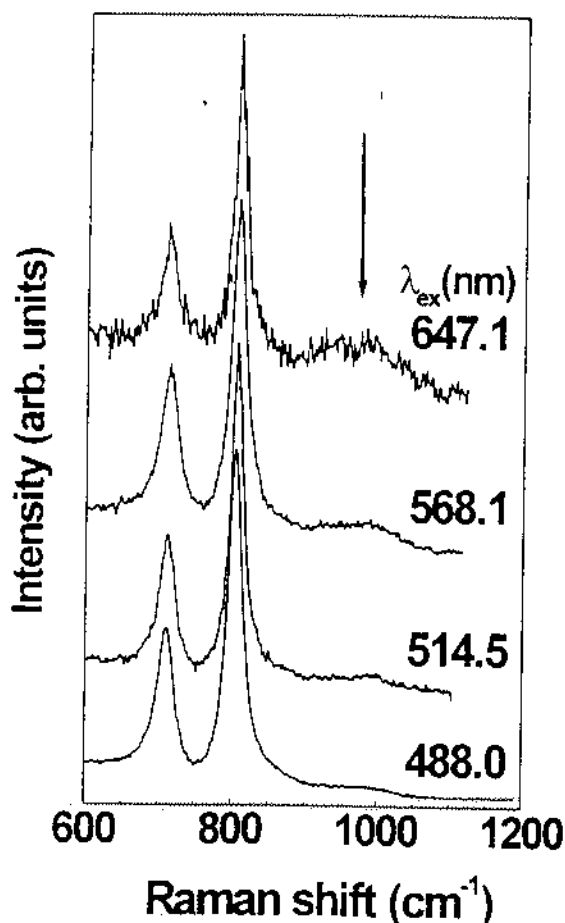
Fig. 7. Raman resonance effect for the band at \sim 970\text{ cm}^{-1} (indicated by arrow) in the mixed sample 0.95\text{ WO}_3 \cdot 0.05\text{ ReO}_2 . All spectra are normalized using the two strongest bands at 700 and 800\text{ cm}^{-1} . The wavelengths of the laser lines, used to excite the spectra, are also shown.
