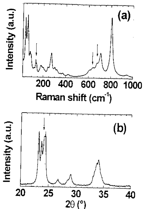
Fig. 3. Raman spectrum (a) and XRD pattern (b) of \text{WO}_3 ground powder after 1h milling. Arrows indicate the typical features of the monoclinic (II) \epsilon -phase: (a) the bands at 143, 643 and 679 \text{ cm}^{-1} and (b) the peak at 2\theta = 24^\circ .
