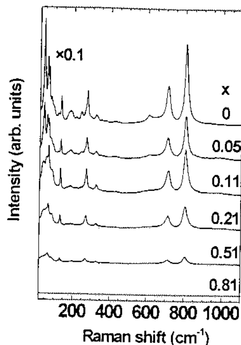
Fig. 6. Raman spectra (excited by the laser line 530.9 nm) of (1-x)\text{WO}_3 \cdot y\text{ReO}_2 mixtures. The intensity of the upper spectrum, corresponding to the treated \text{WO}_3 powder ( x = 0 ) was reduced by a factor 10.
