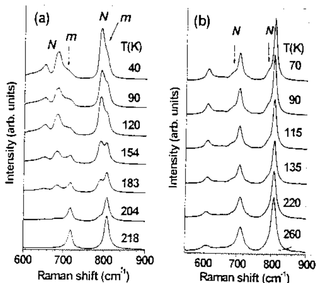
Fig. 4. Low temperature evolution of the high frequency stretching modes in Raman spectra of \text{WO}_3 ; (a) virgin and (b) treated powders. The monoclinic (I) \gamma -phase is labelled by m in (a). Shoulders attributed to the N -phase are indicated in the lowest temperature spectrum in (b). Temperature values are obtained from the Stokes/anti-Stokes ratio in all the cases.
