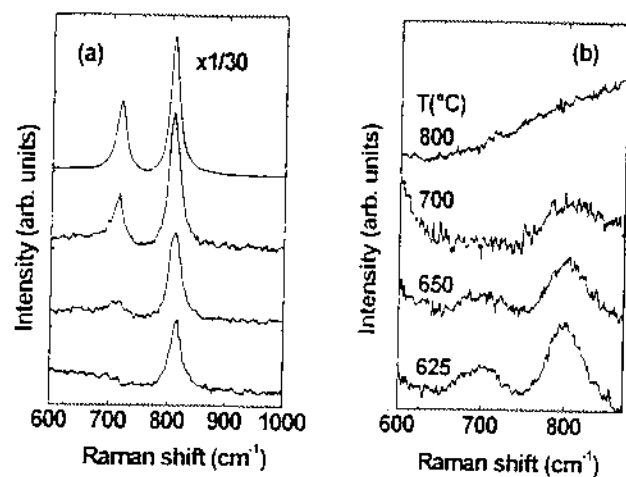
Fig. 1. (a) Evolution of the Raman spectra for H_xWO_3 upon oxidation in air. The starting H_xWO_3 powder with the maximum hydrogen content x = 0.23 is shown at the bottom. The top spectrum, reduced by a factor 30 to be comparable, was obtained after two hours of exposition to air and corresponds to pure monoclinic (I) WO_3 . The intermediate spectra correspond to compositions in the range 0 < x < 0.23 . (b) Temperature dependence of the high frequency Raman modes for the tungsten trioxide WO_3 powder across the orthorhombic-to-tetragonal phase transition.
